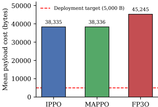
Payload cost vs. deployment target, 5 seeds
